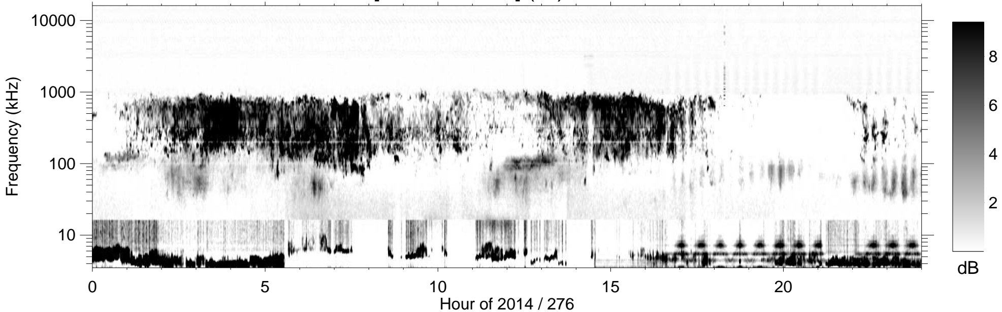
RPWS [ABCH1H2/Ex] (-B) 2014/10/03
