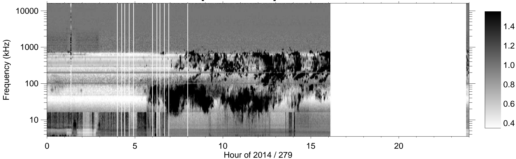
RPWS [ABCH1H2/Ex] (-B) 2014/10/06
