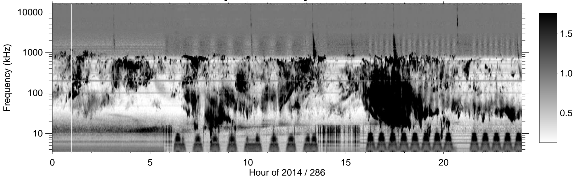
RPWS [ABCH1H2/Ex] (-B) 2014/10/13
