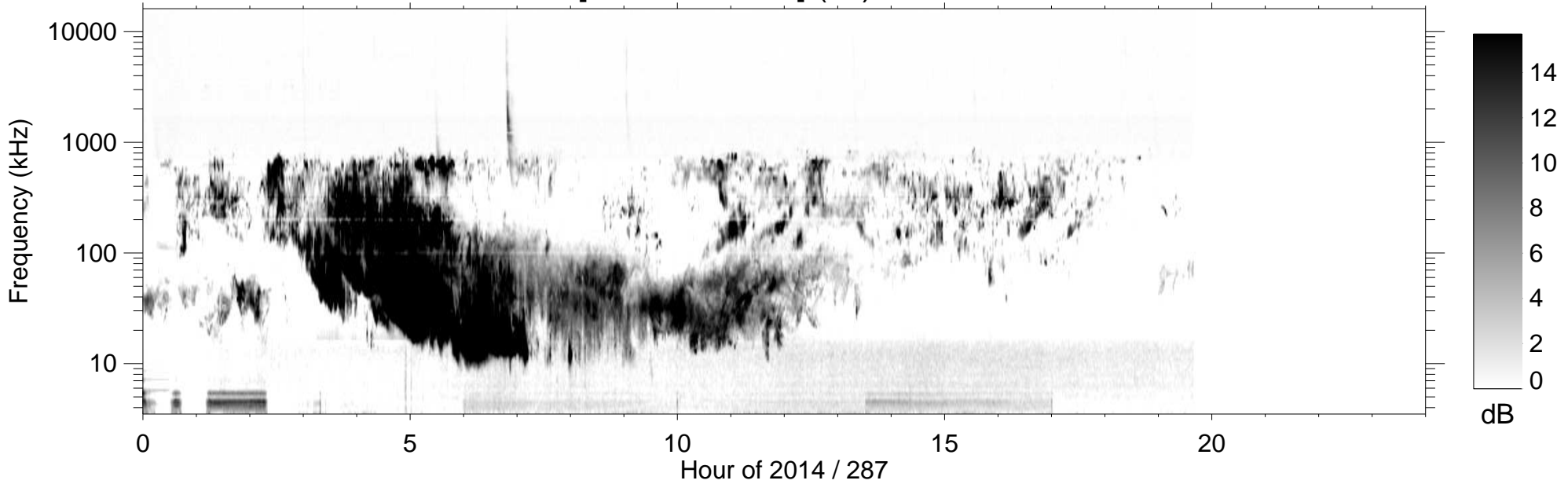
RPWS [ABCH1H2/Ex] (-B) 2014/10/14
