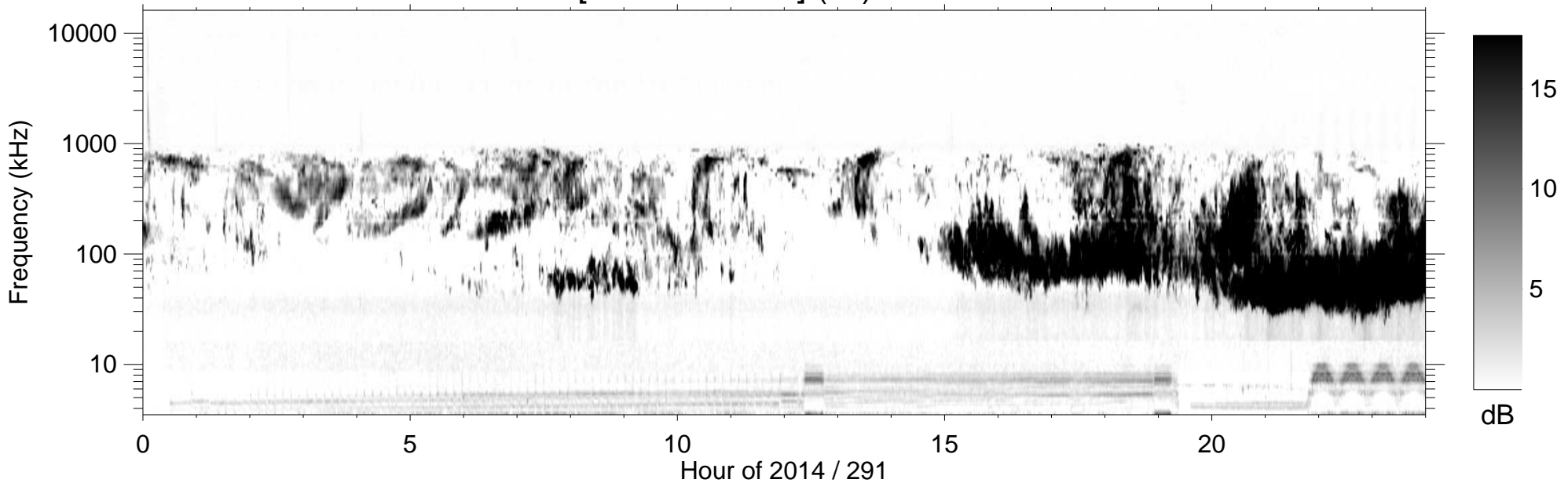
RPWS [ABCH1H2/Ex] (-B) 2014/10/18
