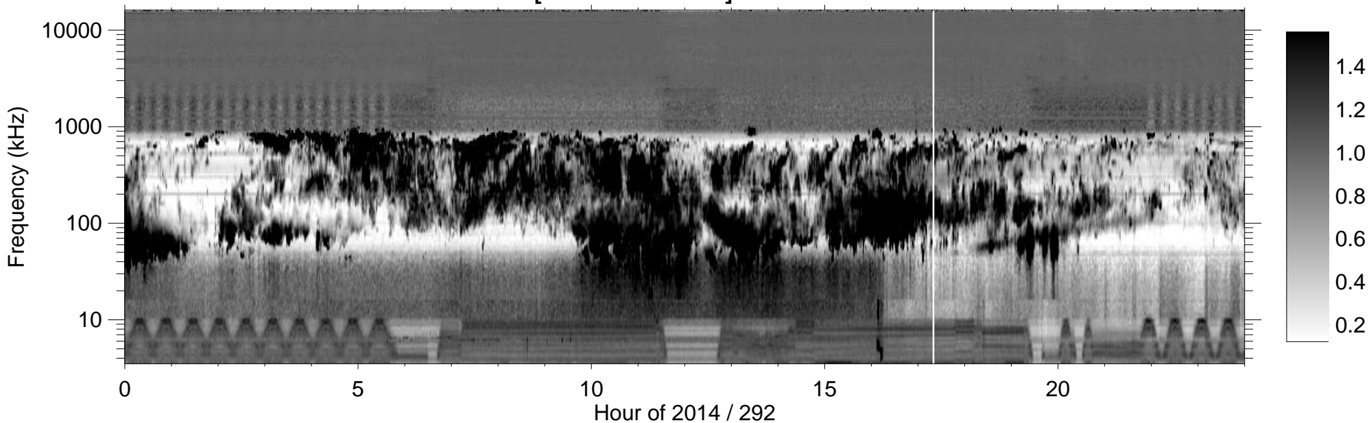
RPWS [ABCH1H2/Ex] (-B) 2014/10/19
