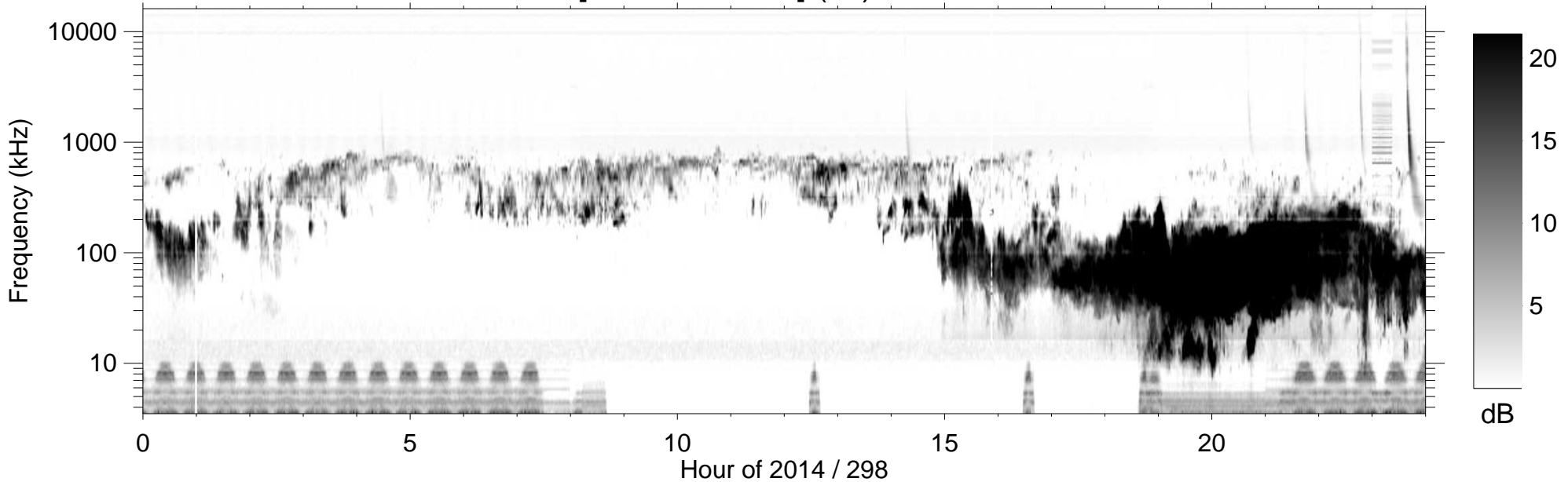
RPWS [ABCH1H2/Ex] (-B) 2014/10/25
