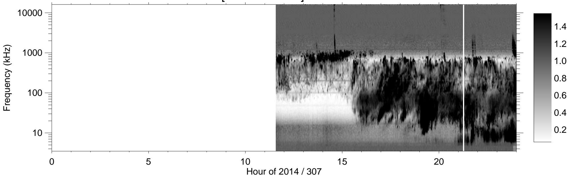
RPWS [ABCH1H2/Ex] (-B) 2014/11/03
