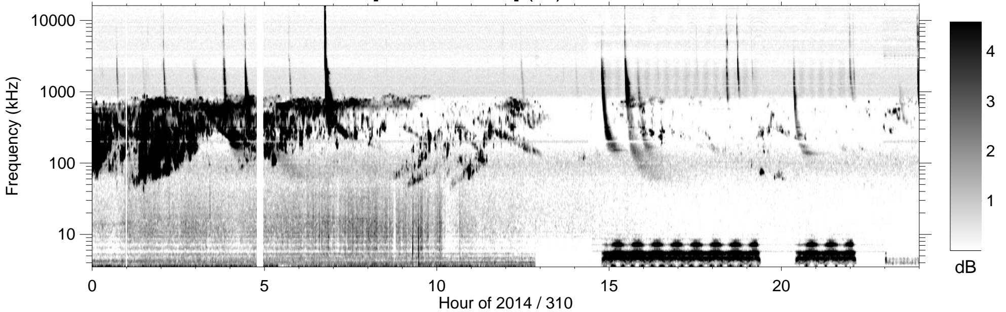
RPWS [ABCH1H2/Ex] (-B) 2014/11/06
