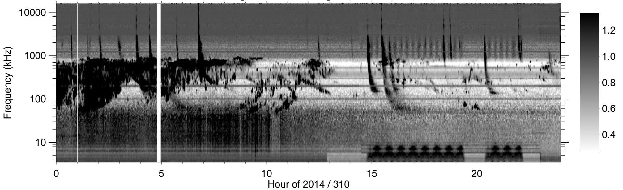
RPWS [ABCH1H2/Ex] (-B) 2014/11/06
