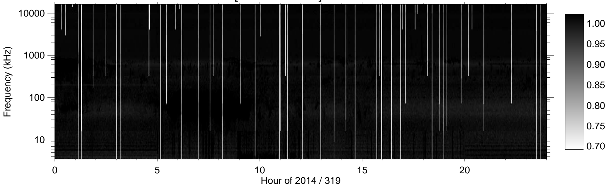
RPWS [ABCH1H2/Ex] (-B) 2014/11/15
