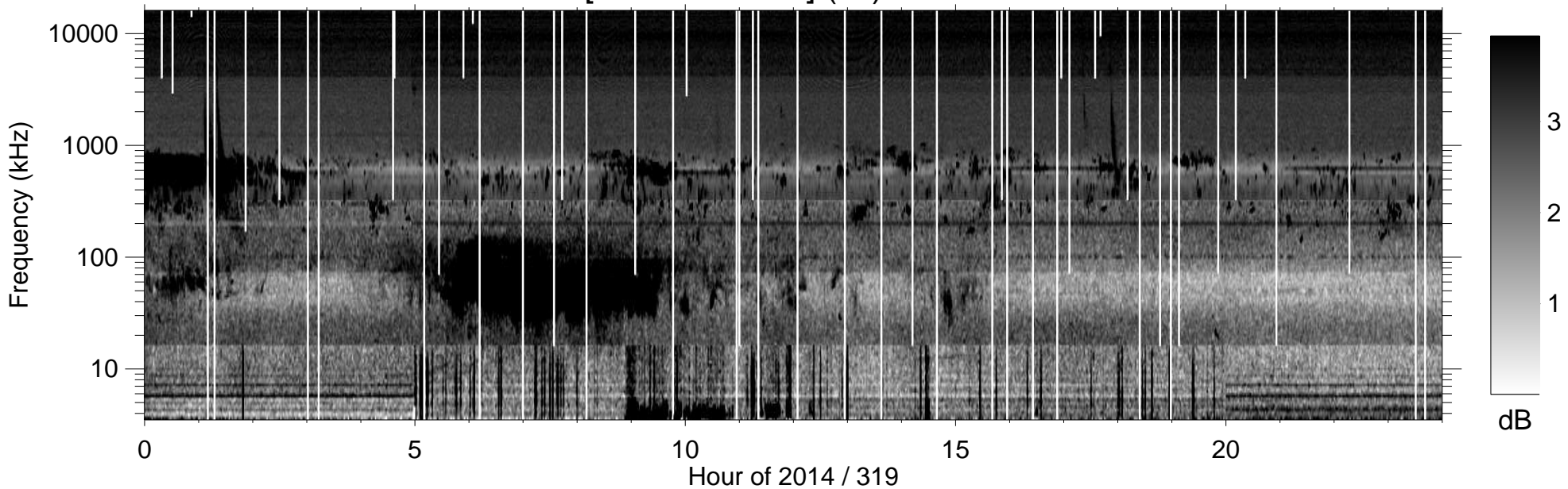
RPWS [ABCH1H2/Ex] (-B) 2014/11/15
