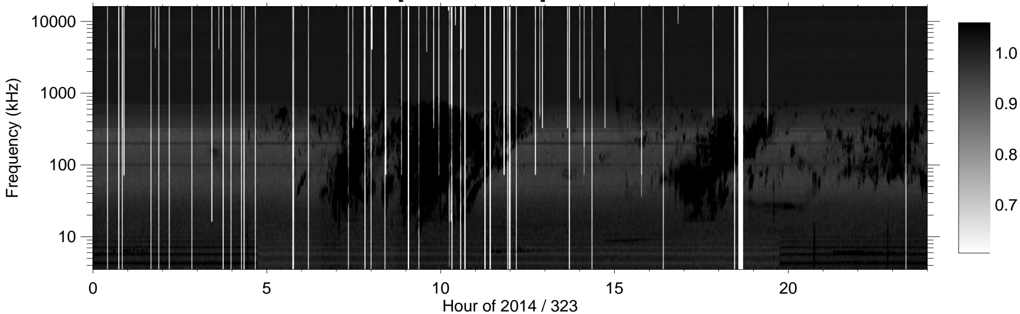
RPWS [ABCH1H2/Ex] (-B) 2014/11/19
