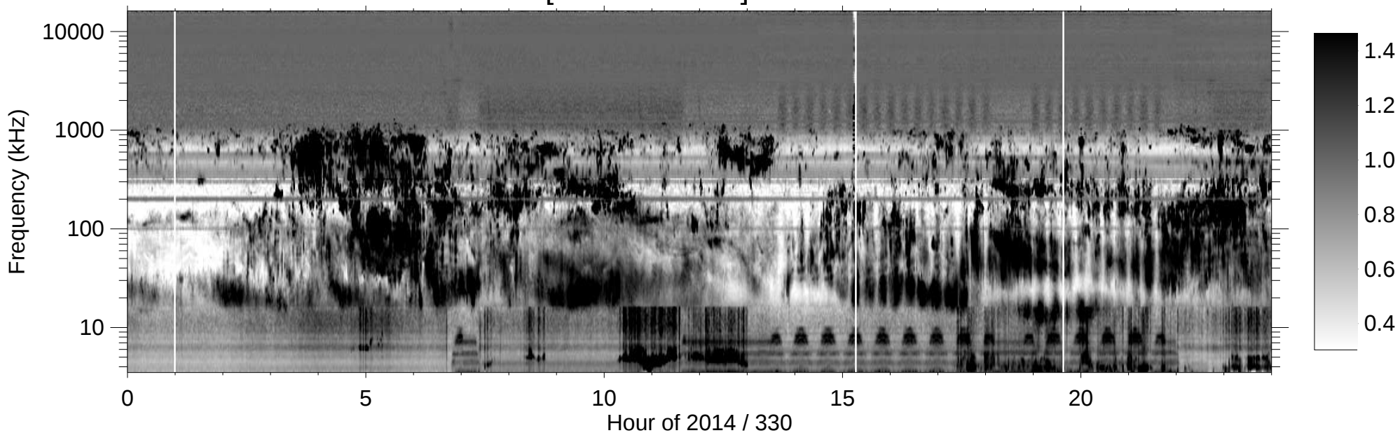
RPWS [ABCH1H2/Ex] (-B) 2014/11/26
