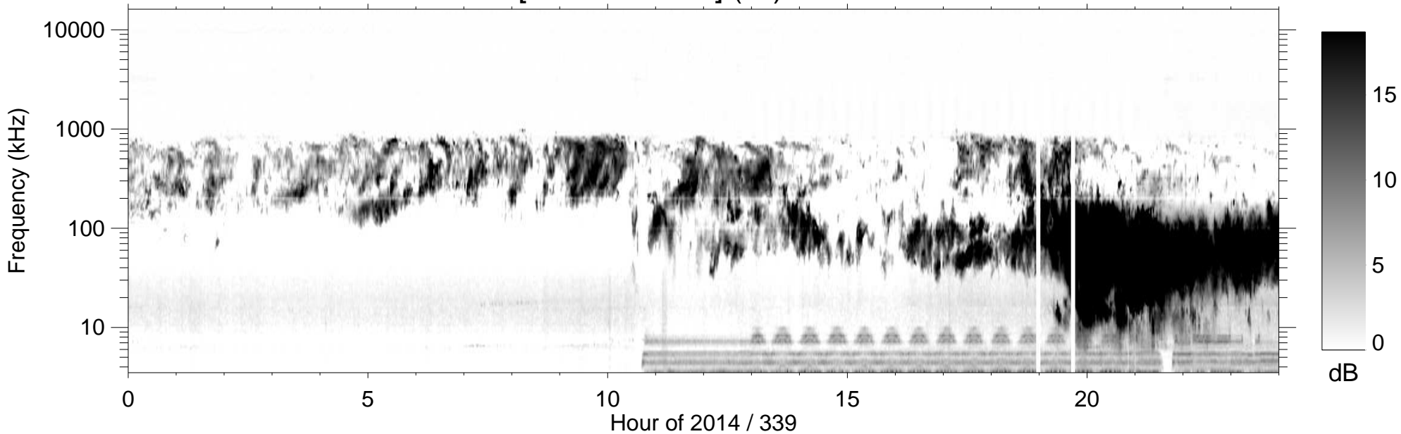
RPWS [ABCH1H2/Ex] (-B) 2014/12/05
