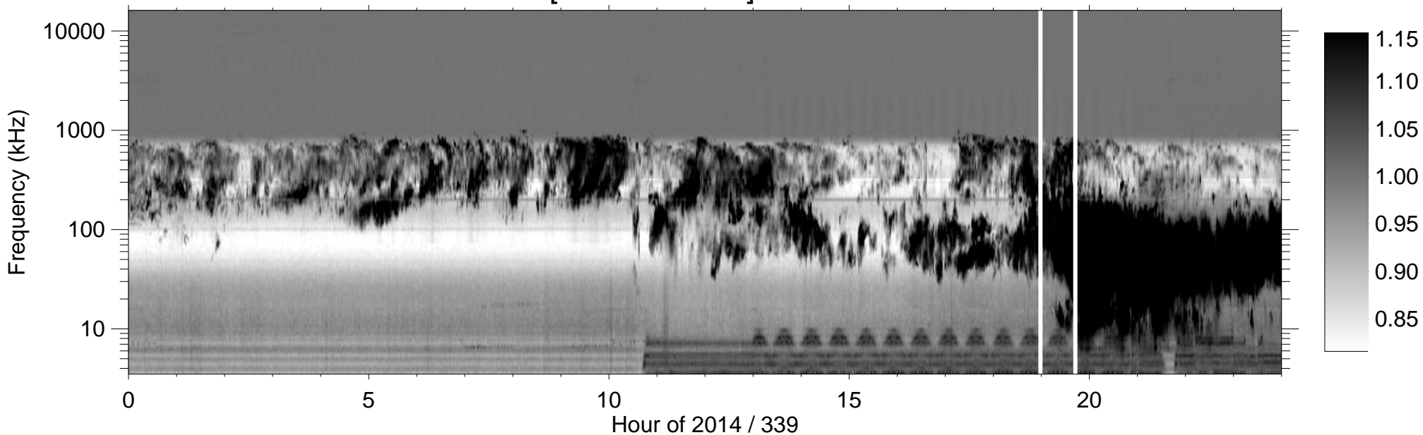
RPWS [ABCH1H2/Ex] (-B) 2014/12/05
