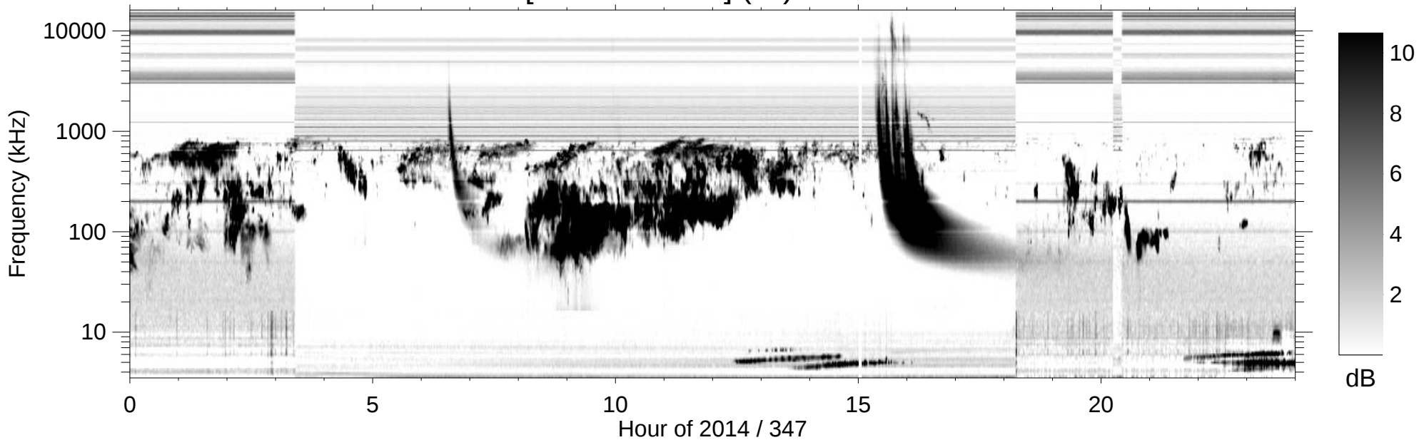
RPWS [ABCH1H2/Ex] (-B) 2014/12/13
