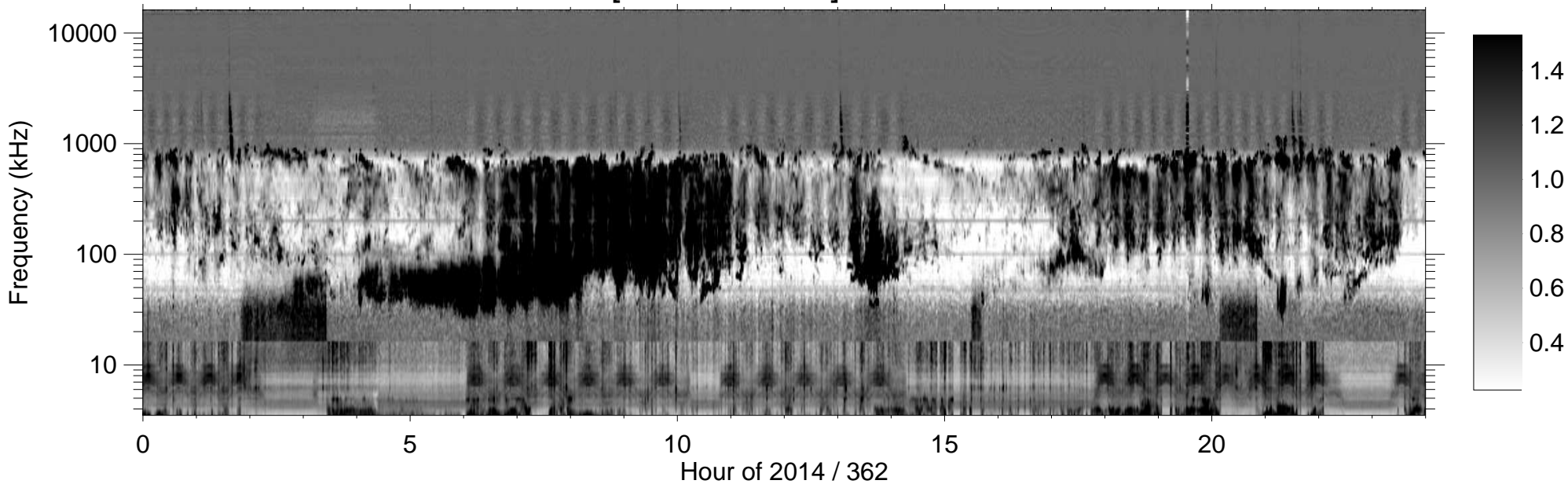
RPWS [ABCH1H2/Ex] (-B) 2014/12/28
