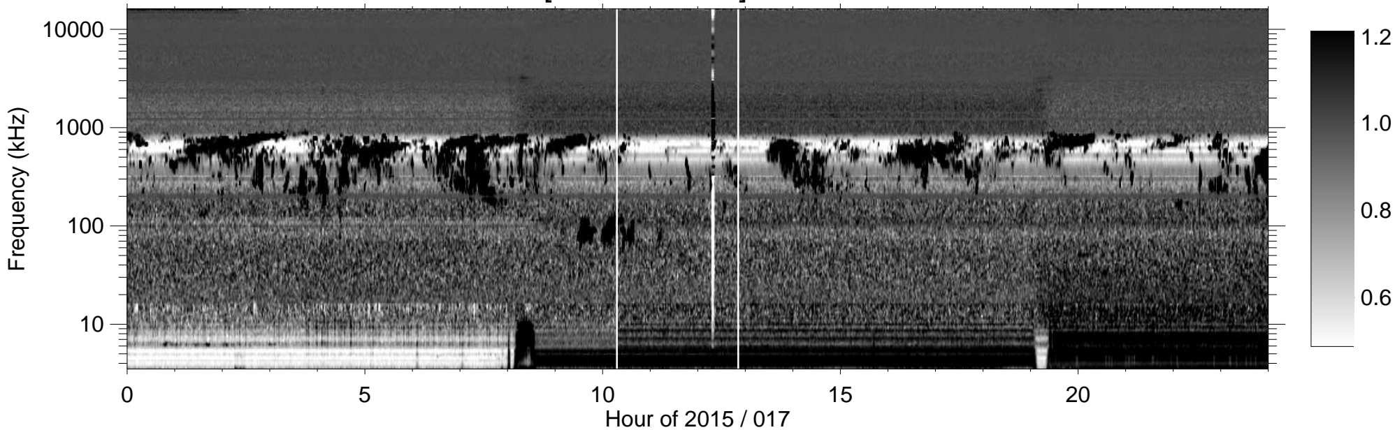
RPWS [ABCH1H2/Ex] (-B) 2015/01/17
