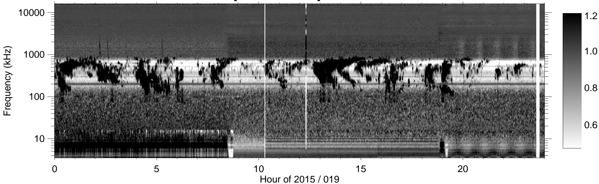
RPWS [ABCH1H2/Ex] (-B) 2015/01/19
