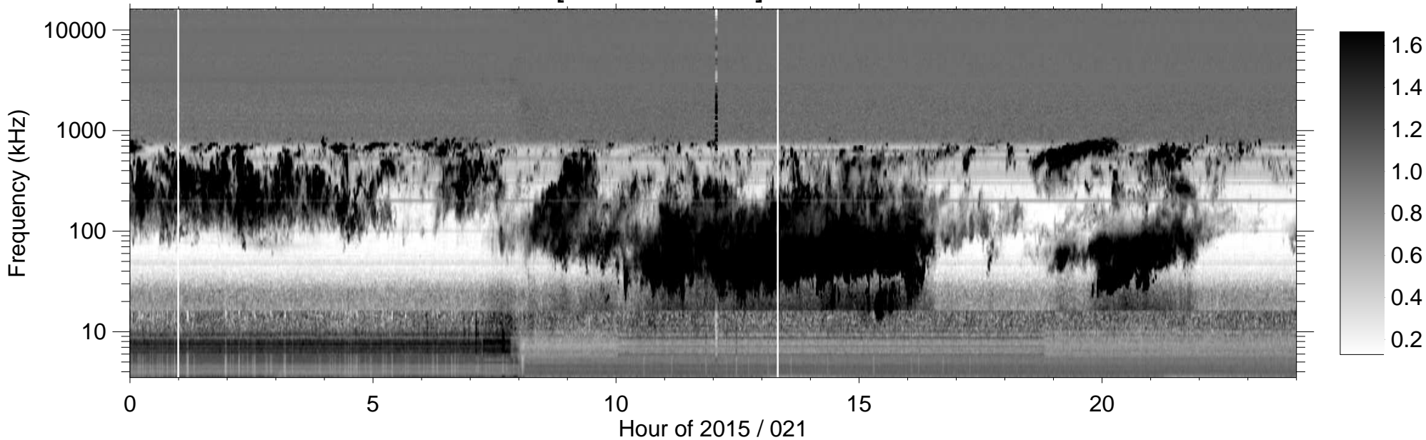
RPWS [ABCH1H2/Ex] (-B) 2015/01/21
