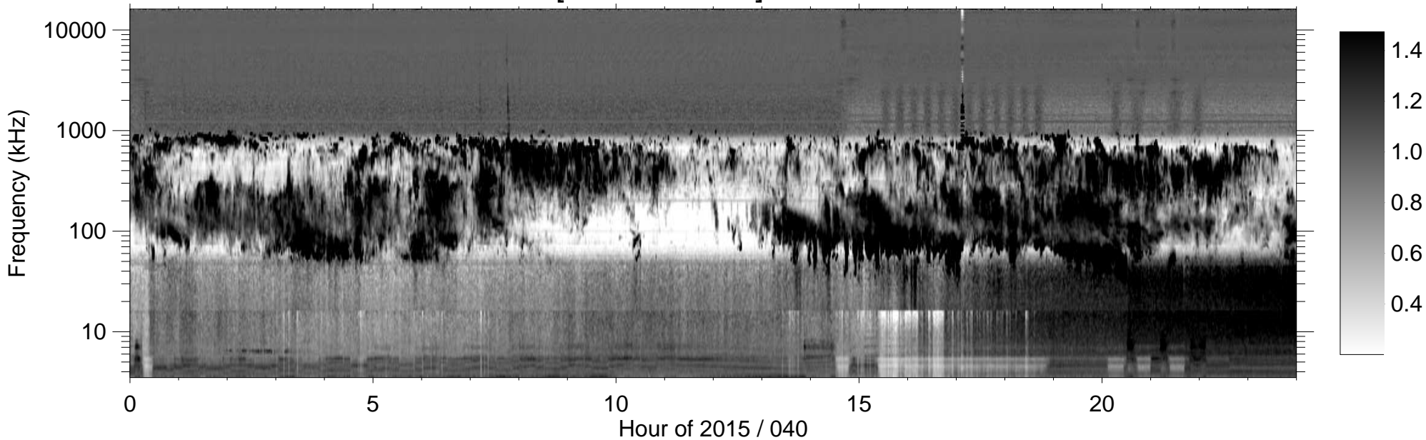
RPWS [ABCH1H2/Ex] (-B) 2015/02/09
