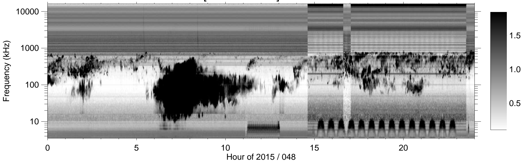
RPWS [ABCH1H2/Ex] (-B) 2015/02/17
