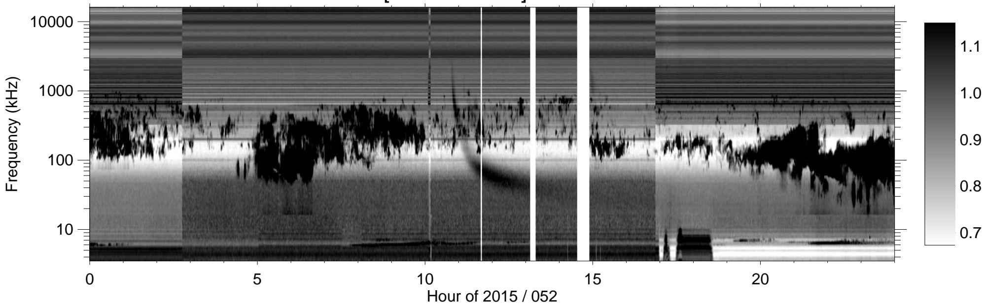
RPWS [ABCH1H2/Ex] (-B) 2015/02/21
