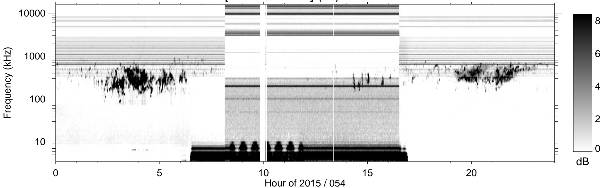
RPWS [ABCH1H2/Ex] (-B) 2015/02/23
