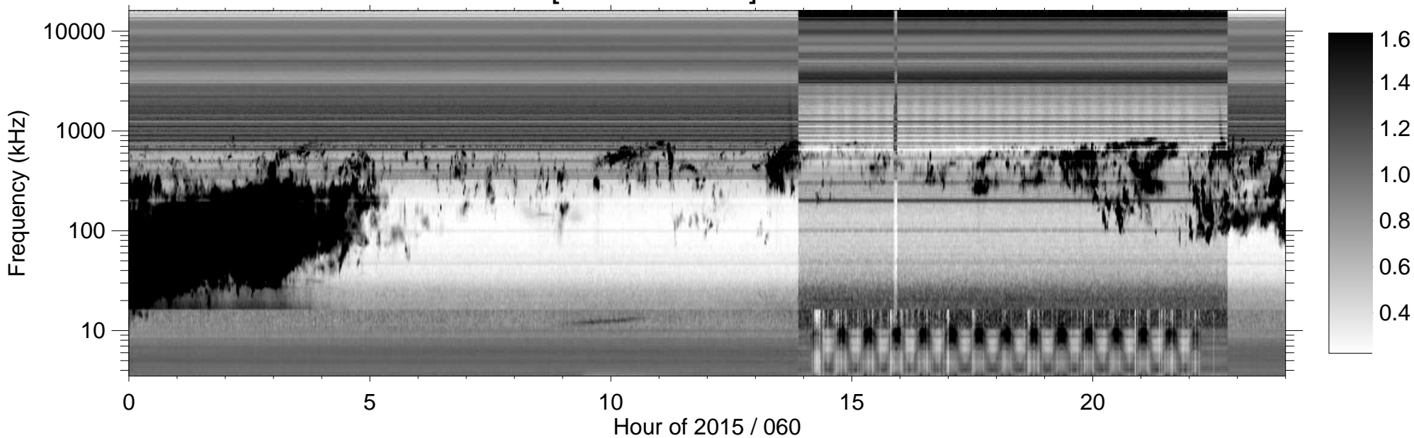
RPWS [ABCH1H2/Ex] (-B) 2015/03/01
