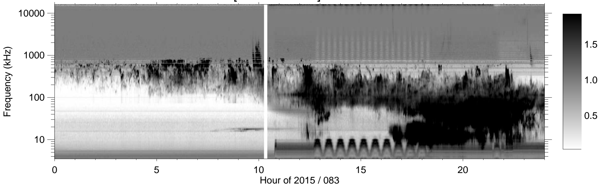
RPWS [ABCH1H2/Ex] (-B) 2015/03/24
