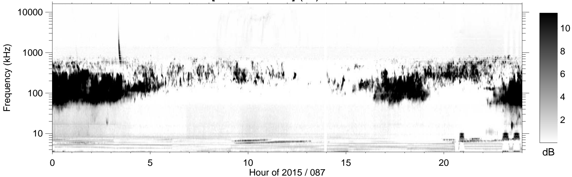
RPWS [ABCH1H2/Ex] (-B) 2015/03/28
