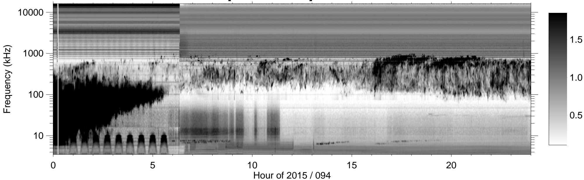
RPWS [ABCH1H2/Ex] (-B) 2015/04/04
