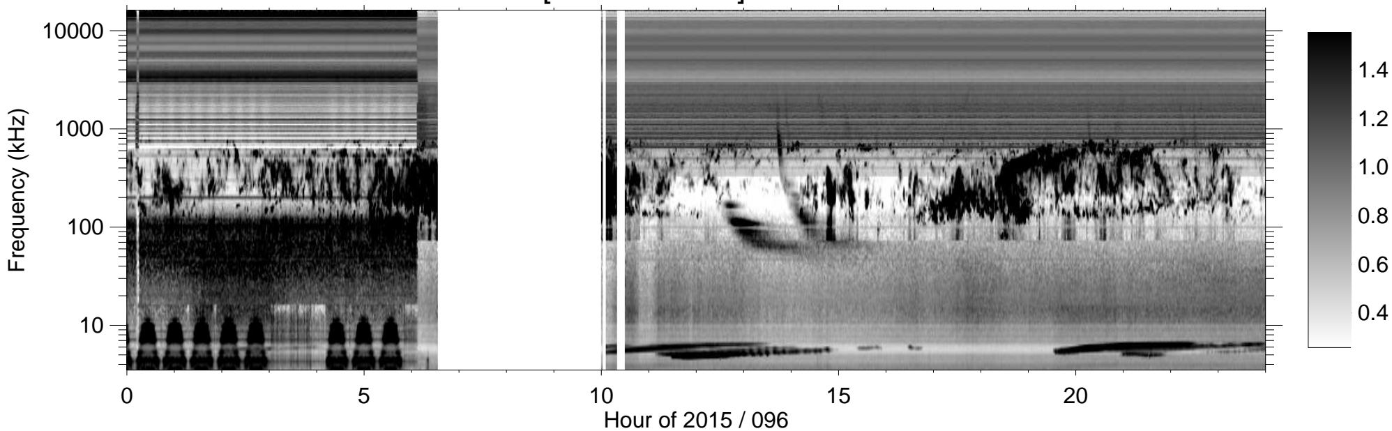
RPWS [ABCH1H2/Ex] (-B) 2015/04/06
