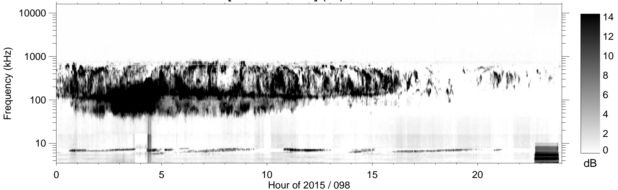
RPWS [ABCH1H2/Ex] (-B) 2015/04/08
