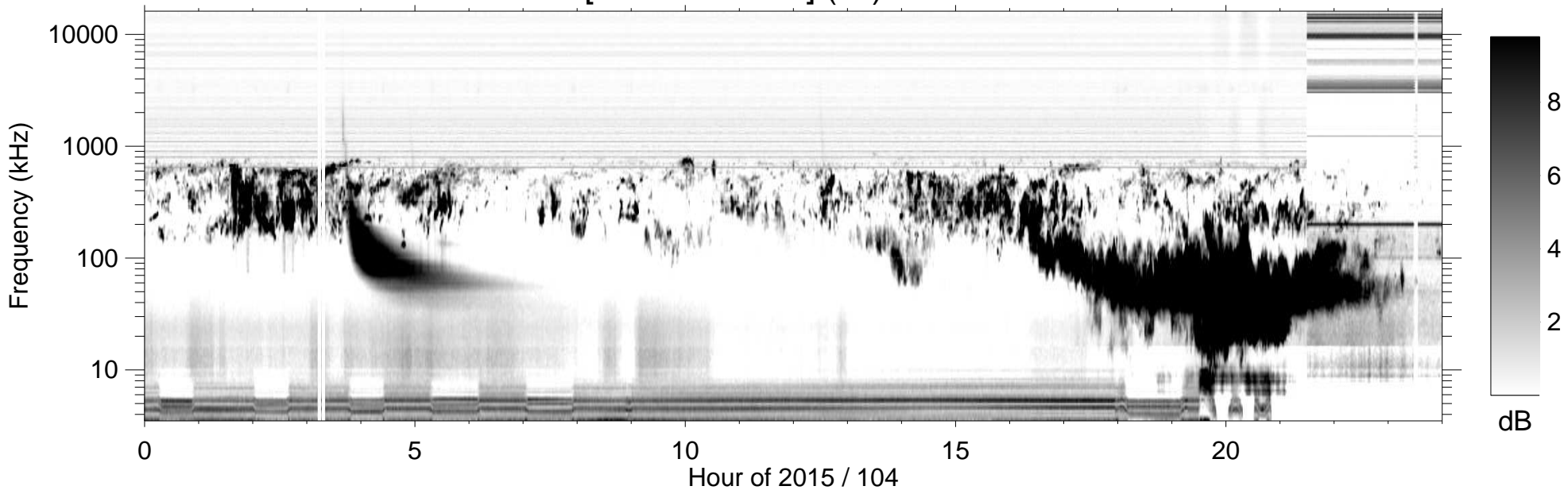
RPWS [ABCH1H2/Ex] (-B) 2015/04/14
