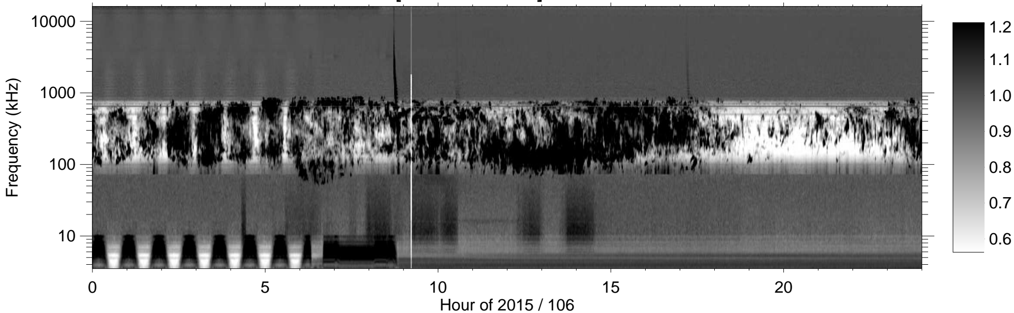
RPWS [ABCH1H2/Ex] (-B) 2015/04/16
