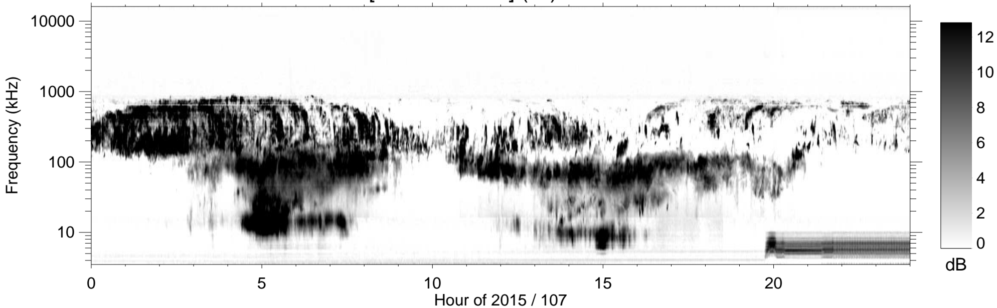
RPWS [ABCH1H2/Ex] (-B) 2015/04/17
