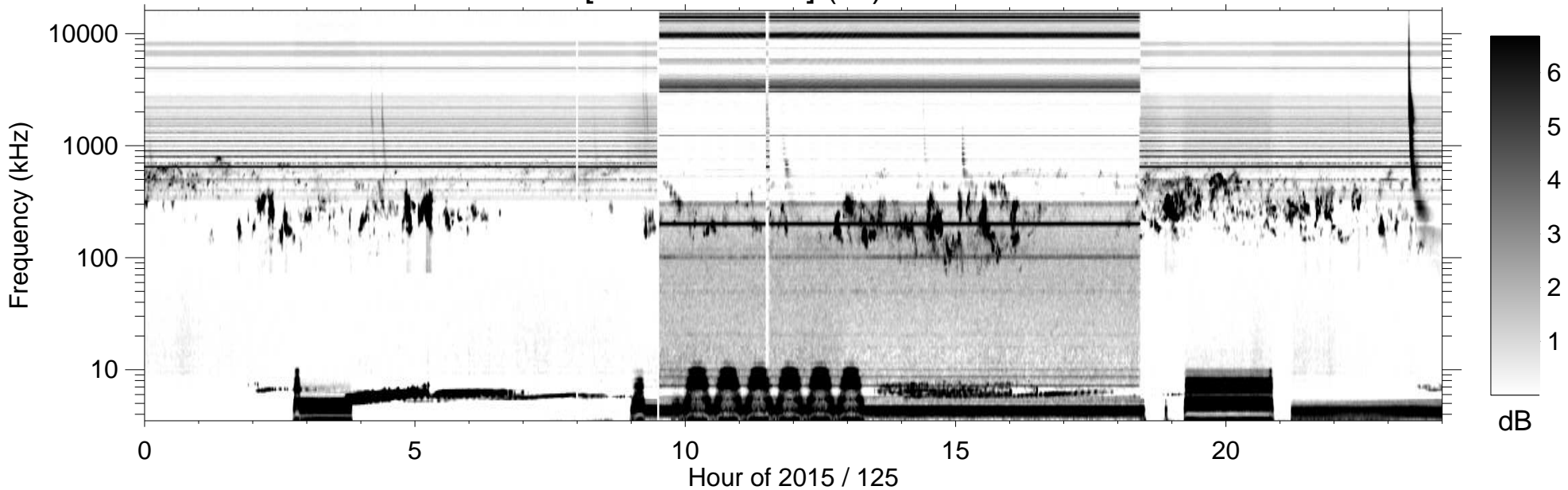
RPWS [ABCH1H2/Ex] (-B) 2015/05/05
