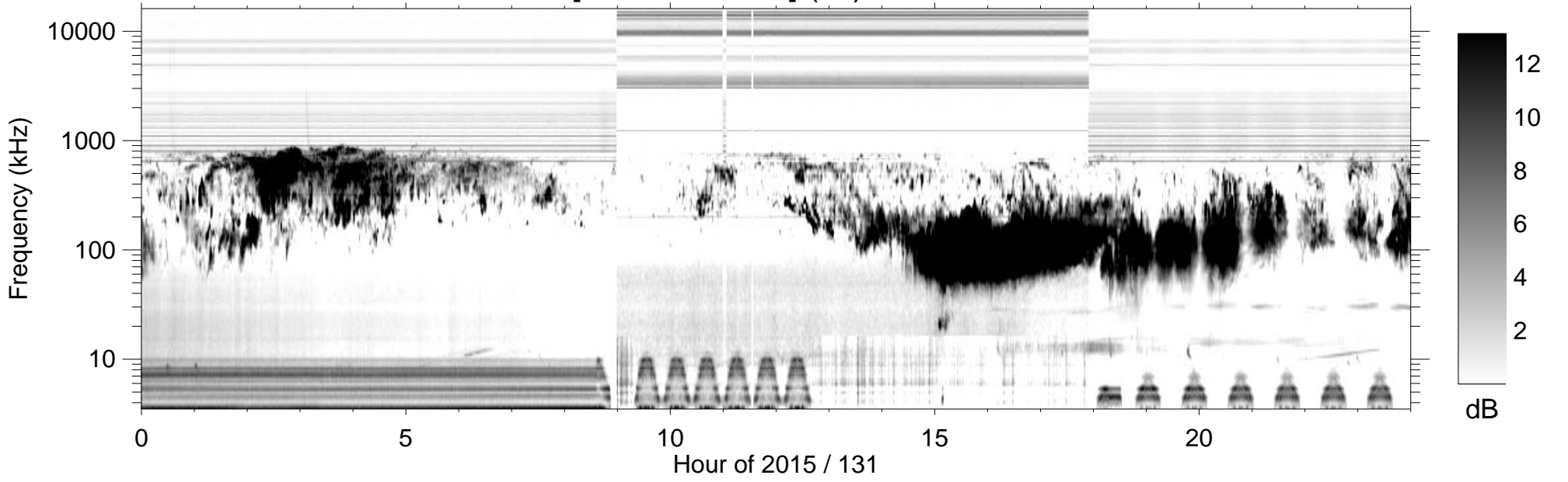
RPWS [ABCH1H2/Ex] (-B) 2015/05/11
