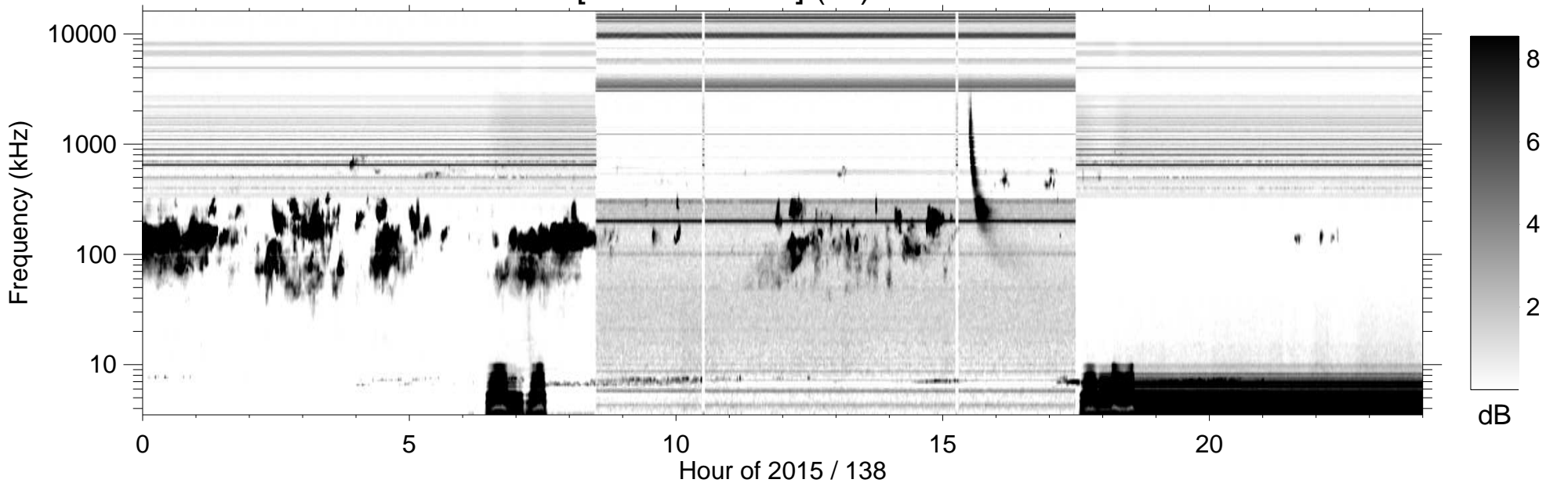
RPWS [ABCH1H2/Ex] (-B) 2015/05/18
