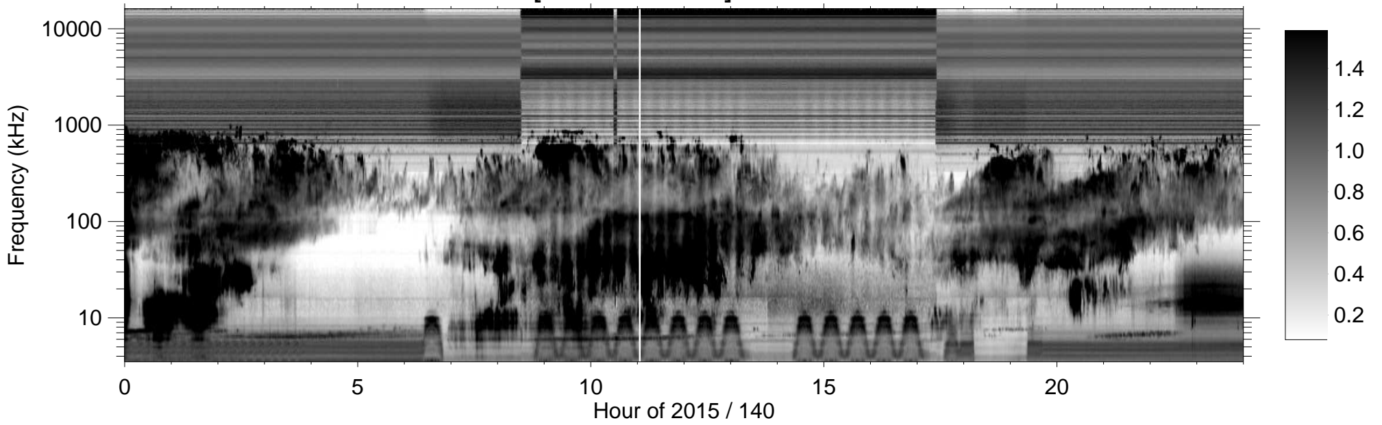
RPWS [ABCH1H2/Ex] (-B) 2015/05/20
