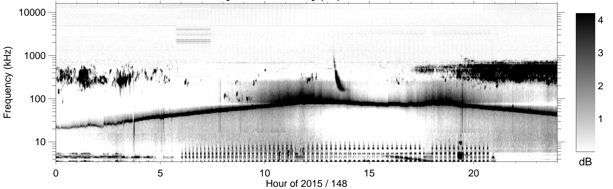
RPWS [ABCH1H2/Ex] (-B) 2015/05/28
