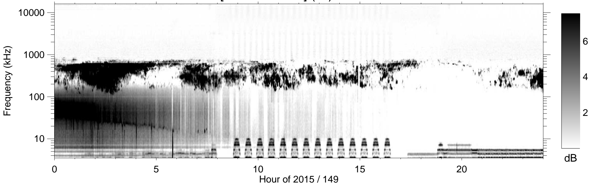
RPWS [ABCH1H2/Ex] (-B) 2015/05/29
