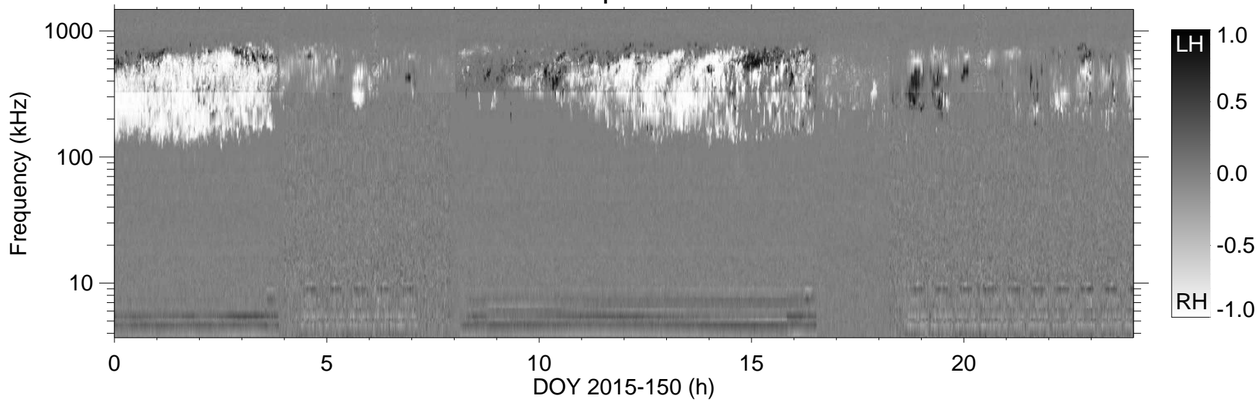
Circular polarization
