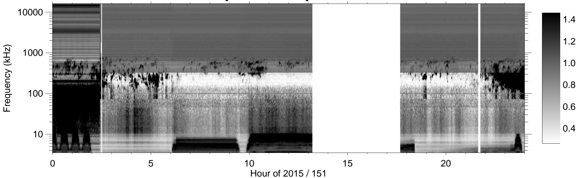
RPWS [ABCH1H2/Ex] (-B) 2015/05/31
