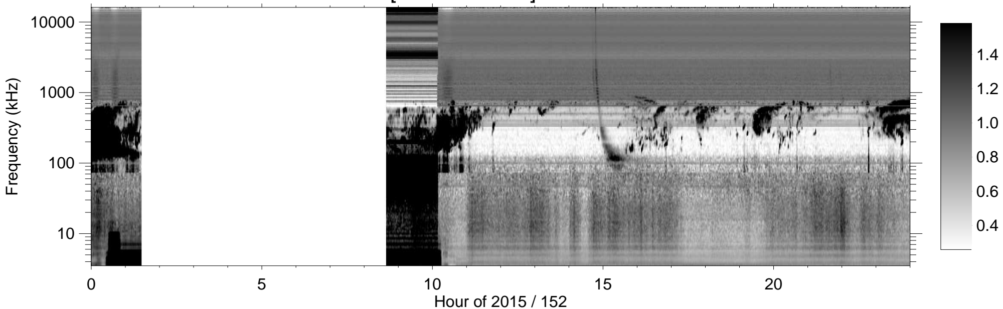
RPWS [ABCH1H2/Ex] (-B) 2015/06/01
