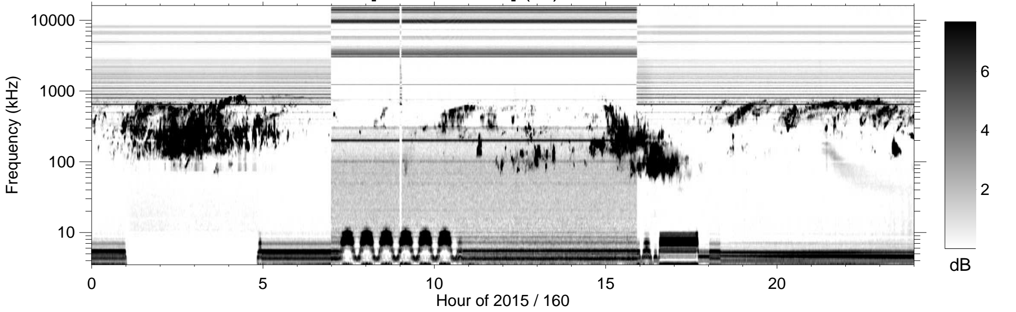
RPWS [ABCH1H2/Ex] (-B) 2015/06/09
