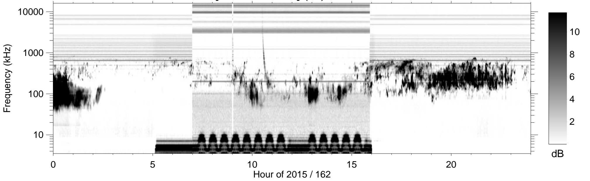
RPWS [ABCH1H2/Ex] (-B) 2015/06/11
