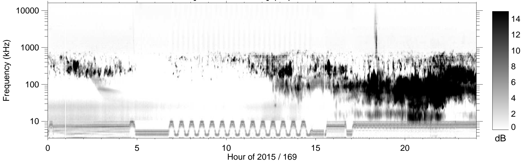
RPWS [ABCH1H2/Ex] (-B) 2015/06/18
