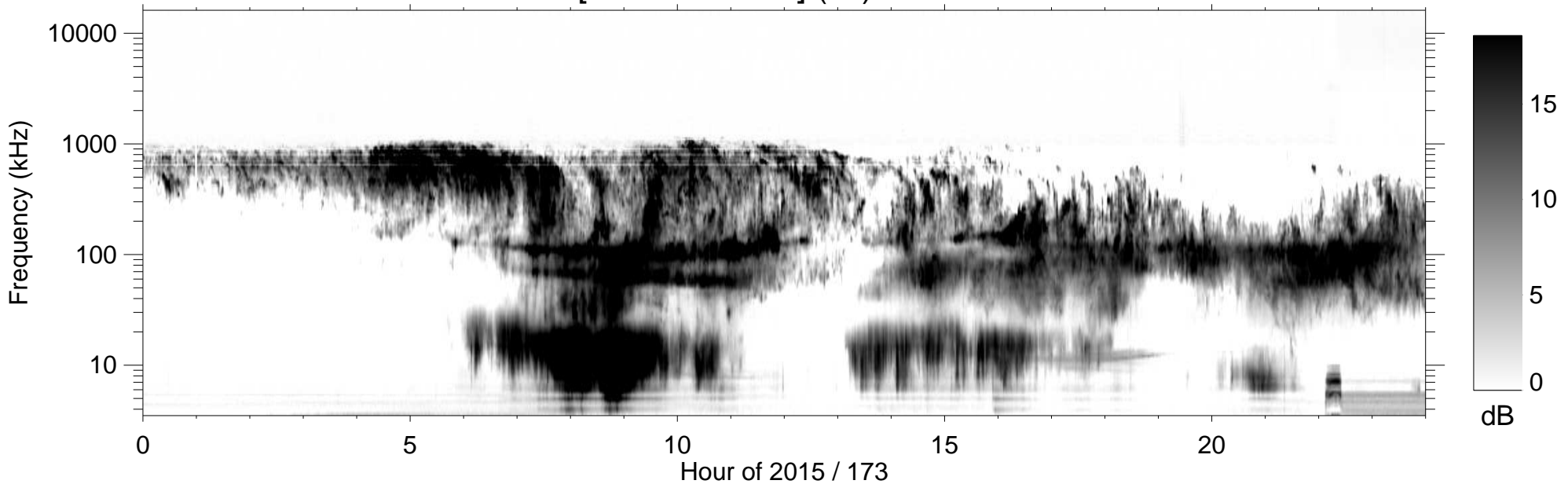
RPWS [ABCH1H2/Ex] (-B) 2015/06/22
