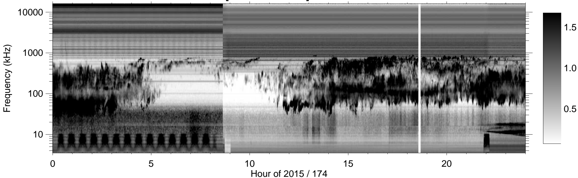
RPWS [ABCH1H2/Ex] (-B) 2015/06/23
