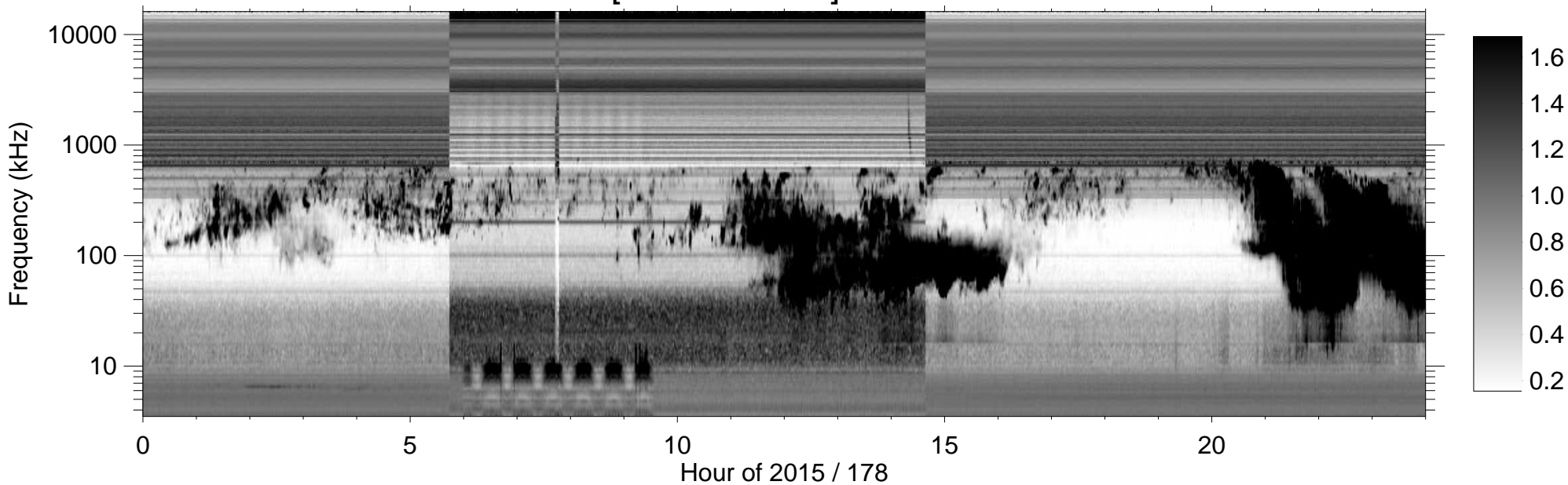
RPWS [ABCH1H2/Ex] (-B) 2015/06/27
