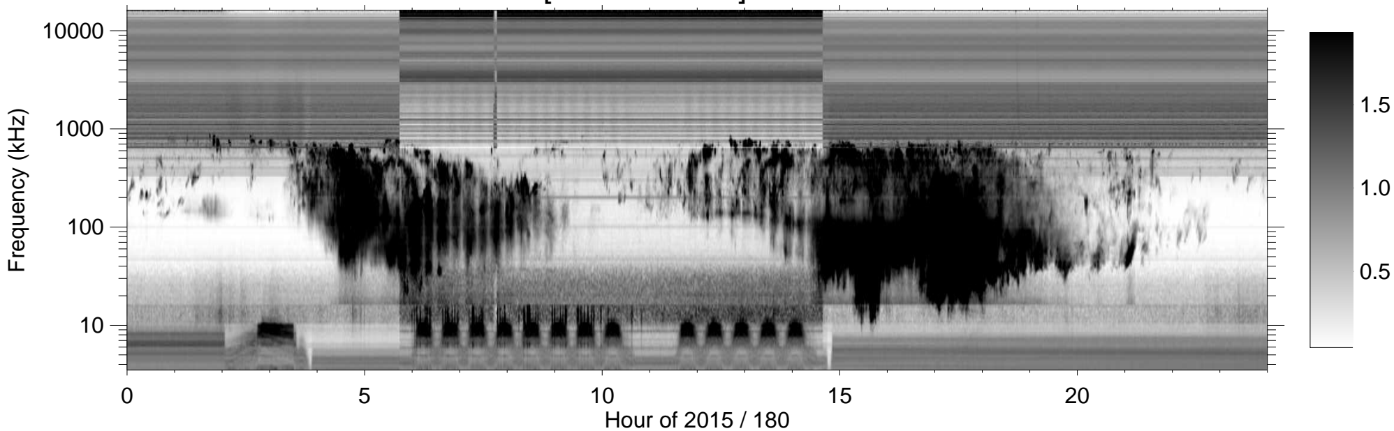
RPWS [ABCH1H2/Ex] (-B) 2015/06/29
