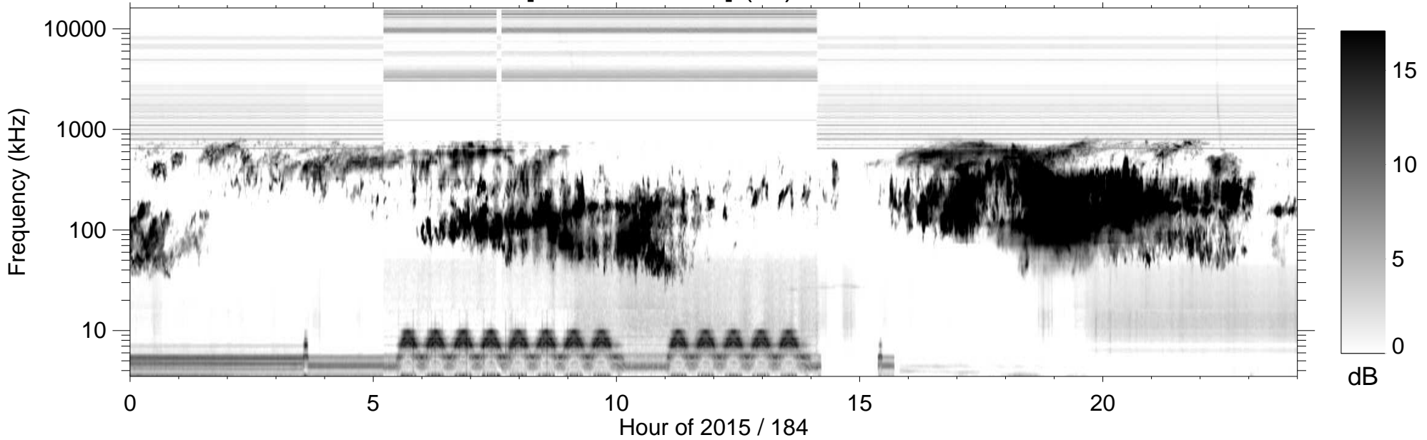
RPWS [ABCH1H2/Ex] (-B) 2015/07/03
