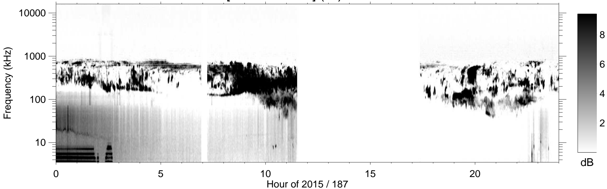
RPWS [ABCH1H2/Ex] (-B) 2015/07/06
