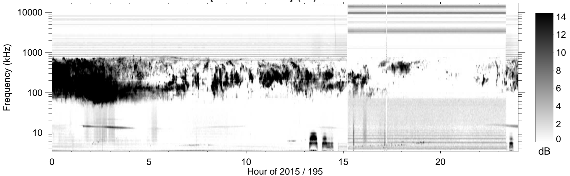
RPWS [ABCH1H2/Ex] (-B) 2015/07/14
